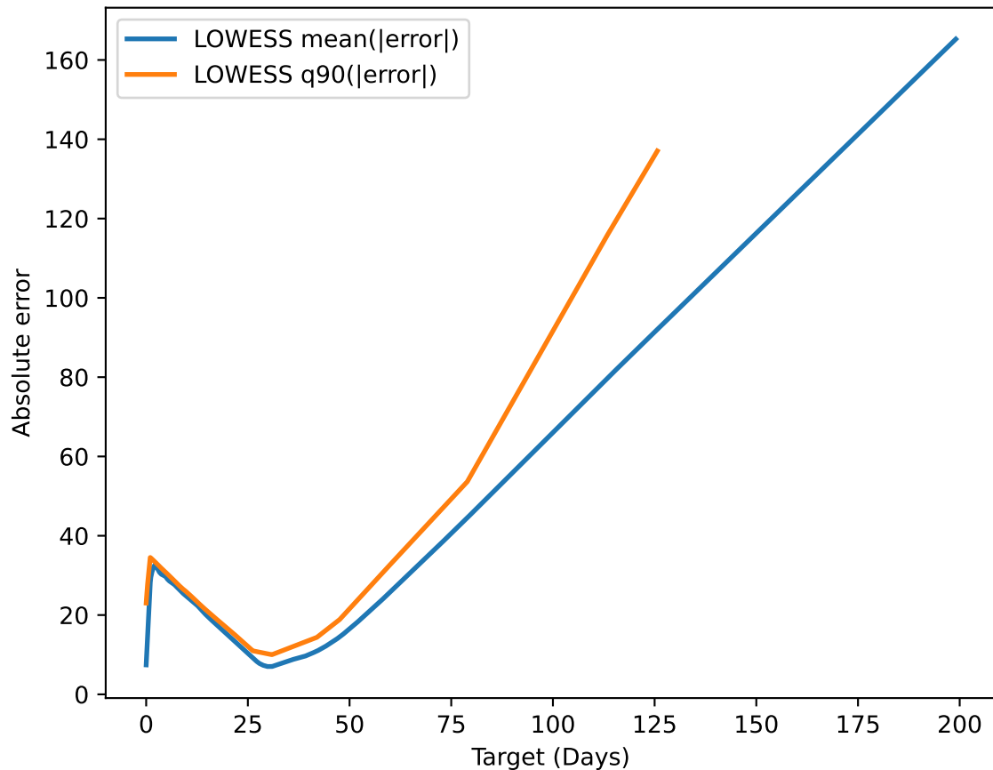
Sepsis: Residual trend vs Target
