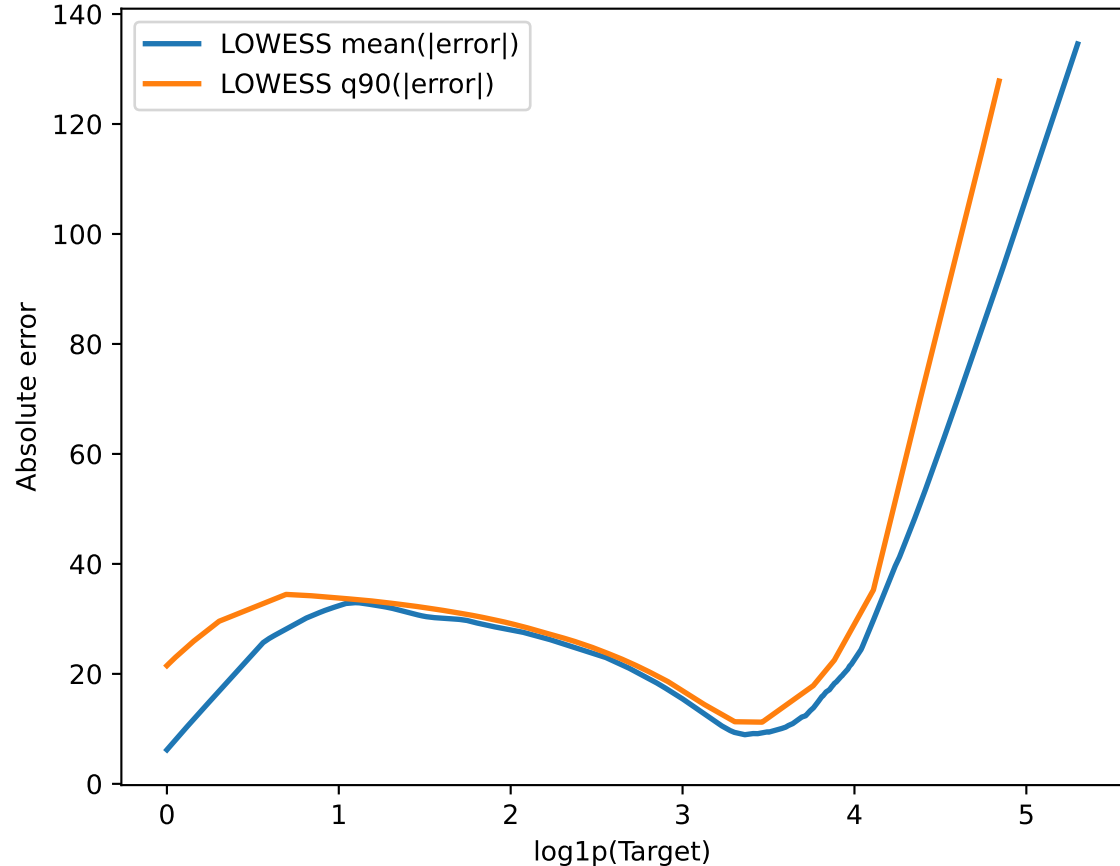
Sepsis: Residual trend vs log1p(Target)
